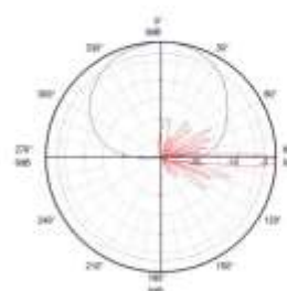
1695–2690 MHz (Ly1/Ry2)
