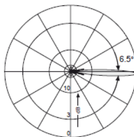
Vertical Pattern 0°–10° electrical downtilt
