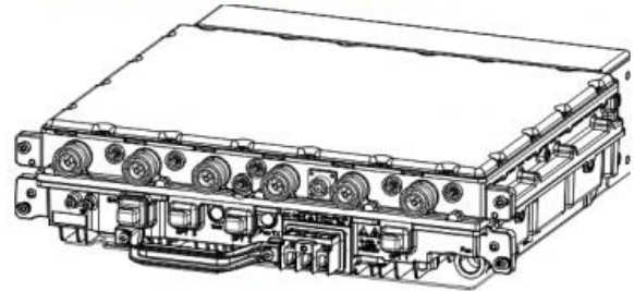
Figure 5 Isometric view of RF Module FRGP
